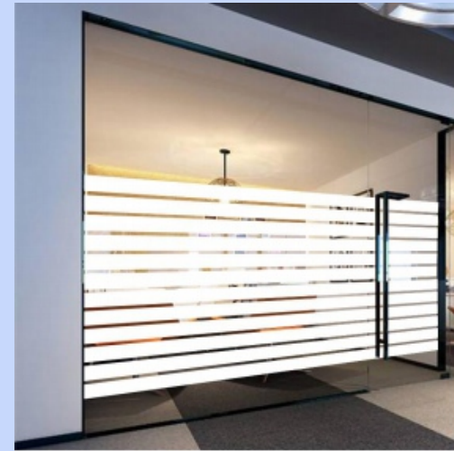
Item No.: SG-210 Material: PET Thickness: 2mil Size: 1.52*30m
